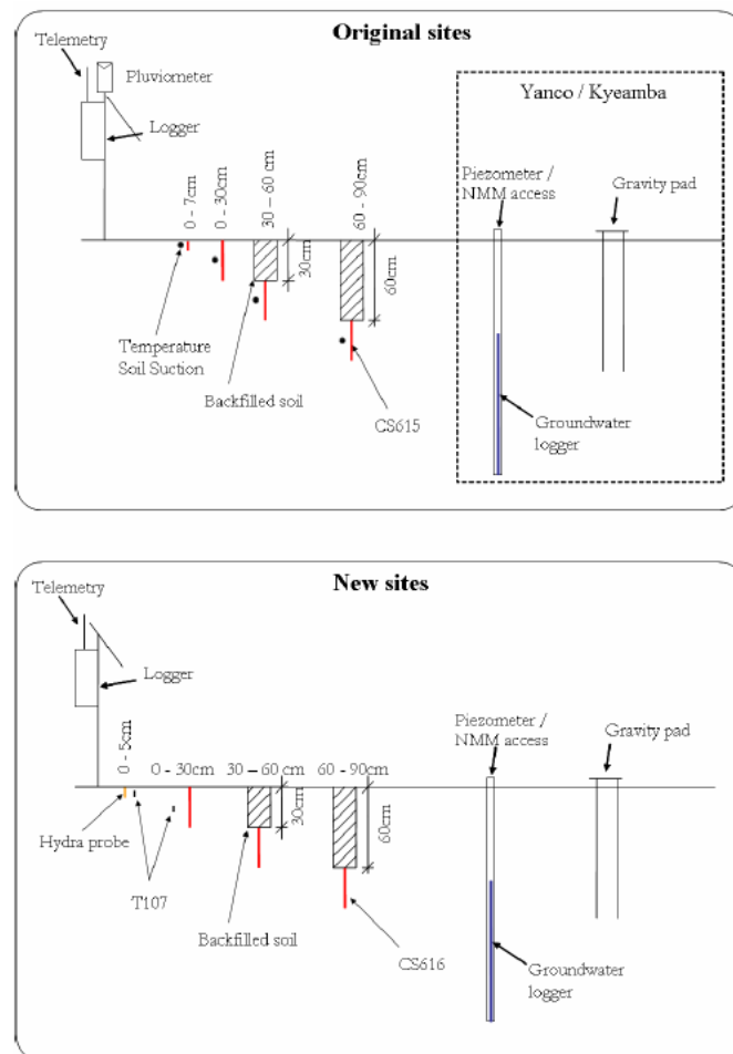
Figure 4-8. Typical equipment at the original (2001) and new (2004) soil moisture sites in the Murrumbidgee catchment. Each site provides continuous data of rainfall, soil moisture at 0- 5 cm (or 0-7 cm), 0-30 cm, 30-60 cm and 60-90 cm and soil temperature and accommodates periodic measurements of gravity, groundwater and TDR soil moisture measurements.
