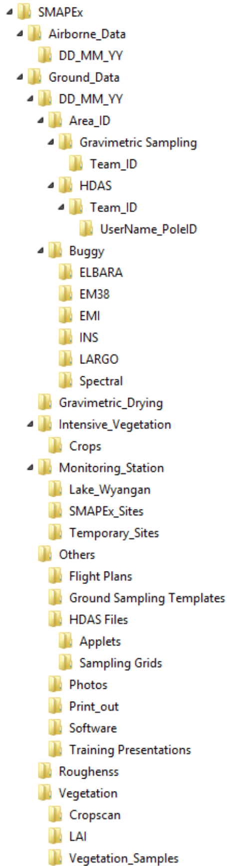
Figure 7-5. Tree diagram of the general SMAPEX-5 file structure.
