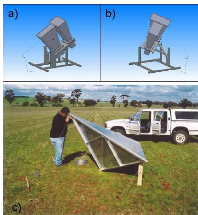
Figure 5-7. Polarimetric Active Radar Calibrators #1 and #2 (a), #3 (b) and Passive Radar Calibrator (c)
