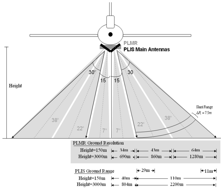
Figure 5-1. Cross-section of PLMR and PLIS viewing configuration on the aircraft.
