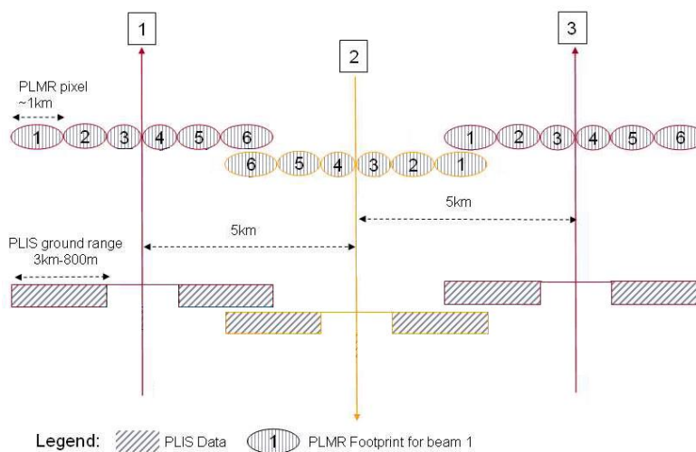
Figure 5-2. Plan view of PLMR and PLIS viewing configuration on the aircraft.
